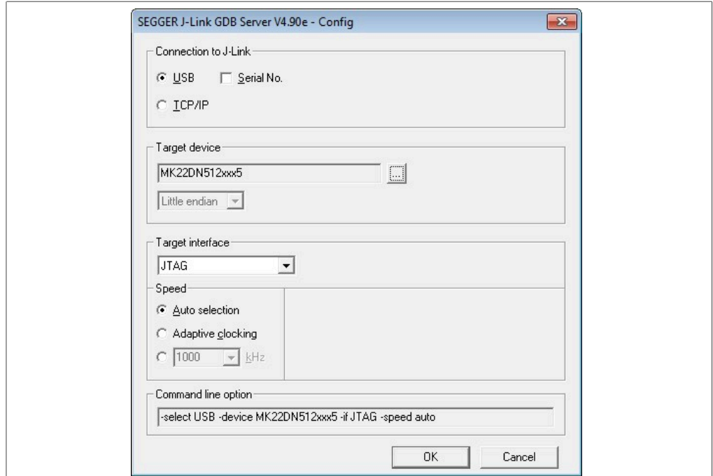
Figure 20. SEGGER J-Link GDB Server configuration
