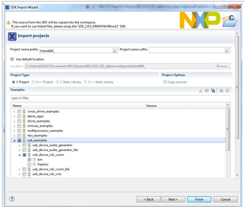
Figure 6. Import project
