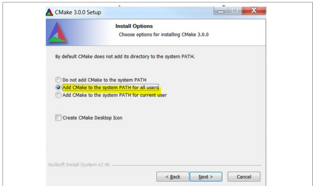
Figure 18. Install CMake
